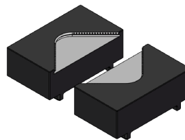
B05 - Profile - V-Shape with Teeth
